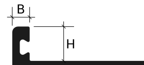
Aluminium TR60 B = 3 mm
